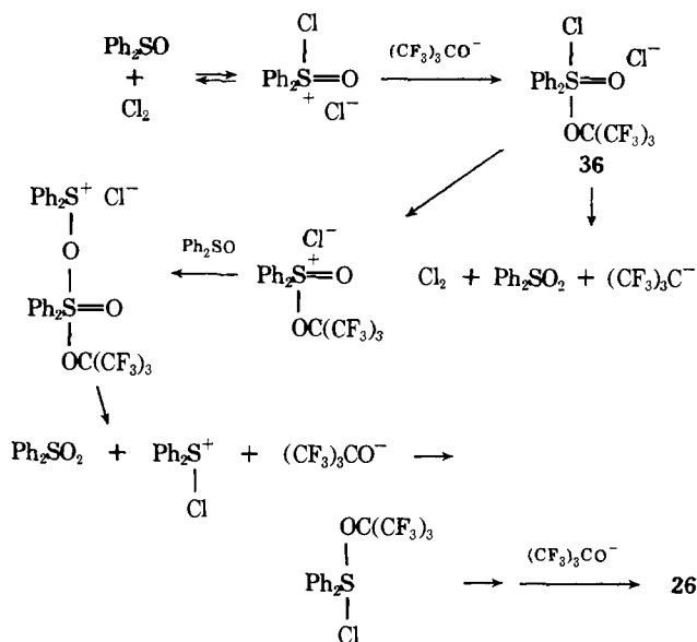
Scheme VIII
