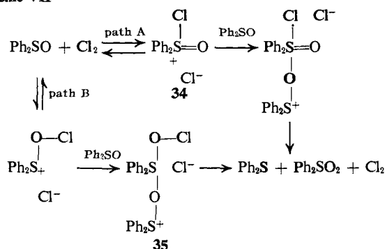
Scheme VII
