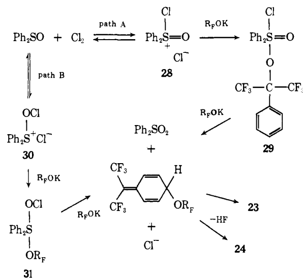
Scheme V
